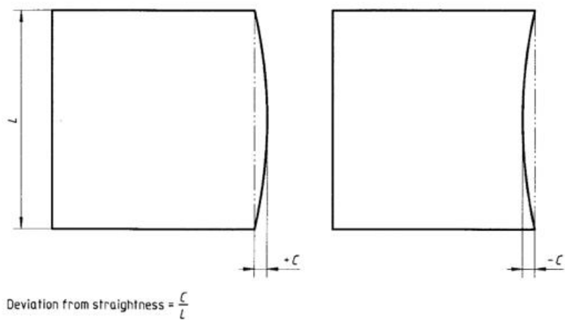
Figure 2 — Straightness of sides
