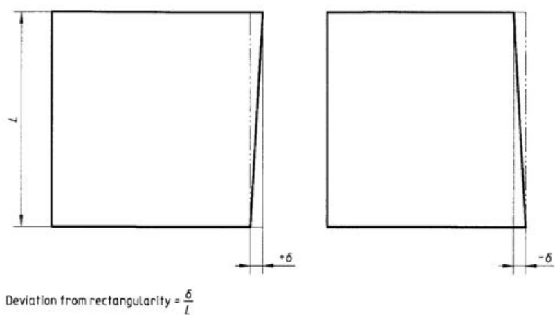
Figure 3 — Rectangularity
