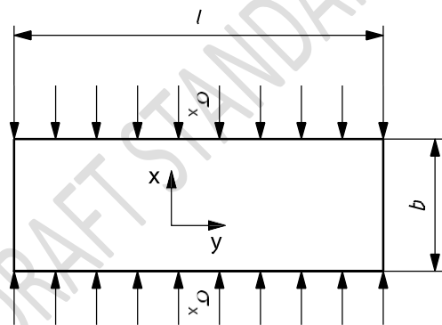
b) Deck compressive stress parallel to small edge of panel (transversal framing)
