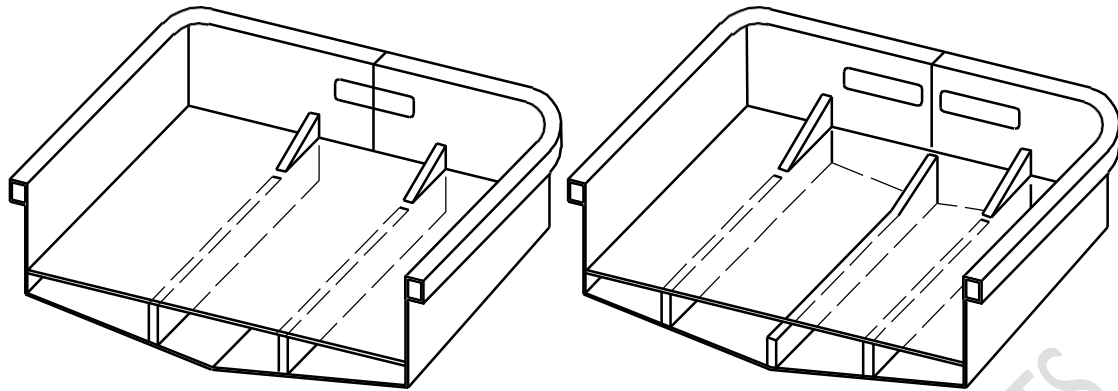
a) Transom reinforced by two bottom girders for single engine
