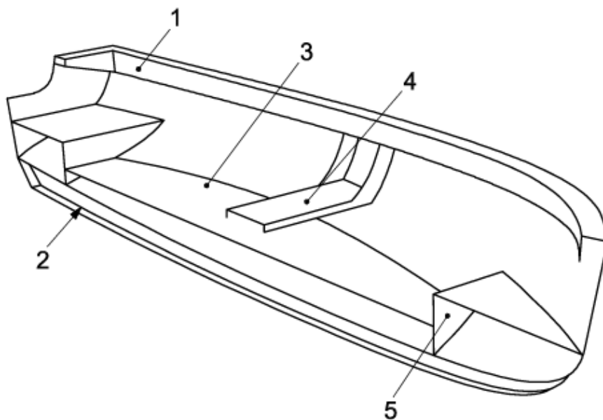
Figure 2: Transversally framed boat
