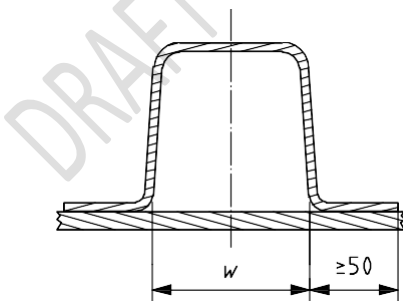
d) Typical boatbuilder's tabbing
