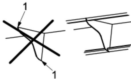
a) Bracket, poor practice and good practice solution
