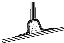
a) Tabbing on both sides only
