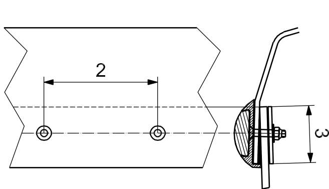
a) Vertical joint
