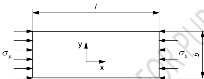
a) Deck compressive stress parallel to long edge of panel (longitudinal framing)
