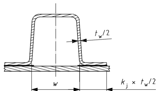
d) Typical glued stiffener
