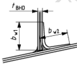
a) Tabbing on both sides only
