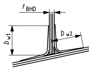
b) Thicker tabbing on one side
