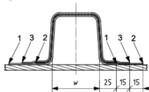
b) Staggered tabbing
